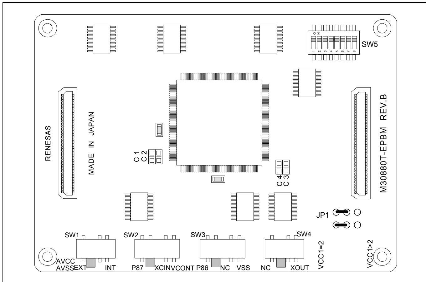
Figure 2.16 Positions of the switches
